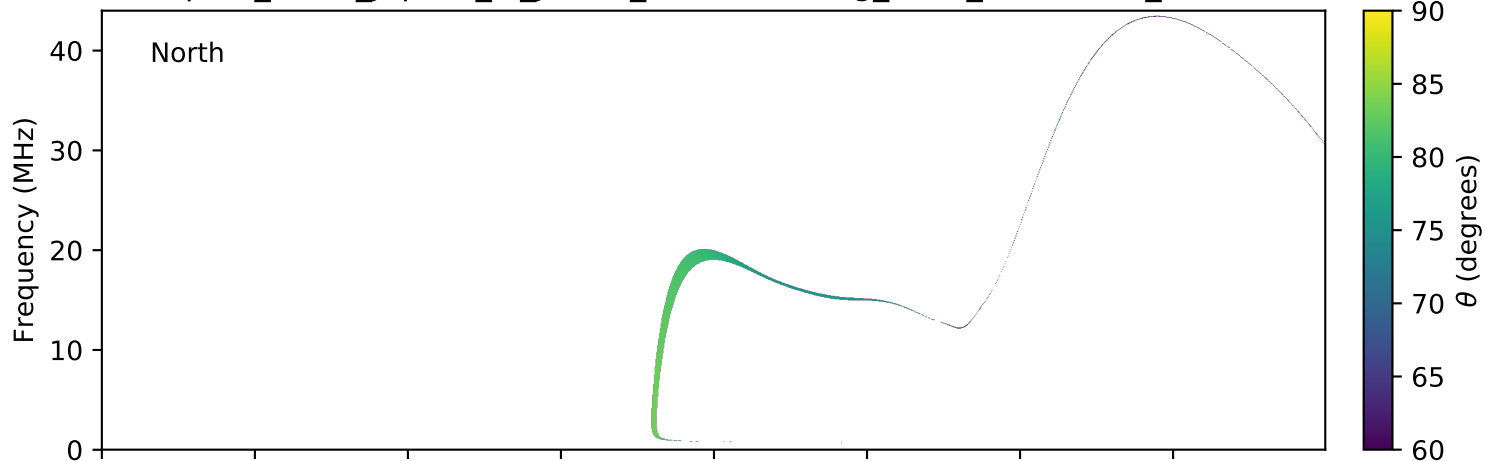
expres_earth_jupiter_io_jrm09_lossc-wid1deg_3kev_20060214_v01.cdf
