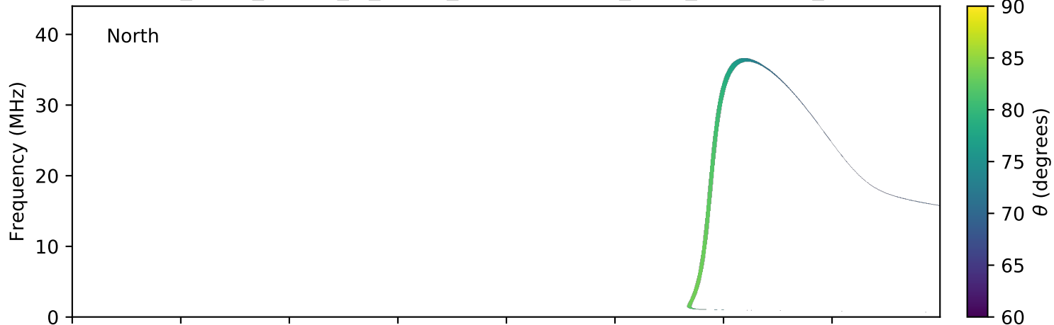
expres_earth_jupiter_io_jrm09_lossc-wid1deg_3kev_20060212_v01.cdf
