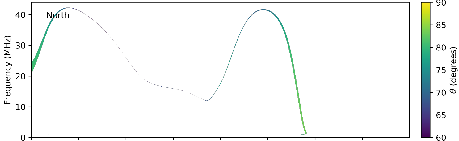
expres_earth_jupiter_io_jrm09_lossc-wid1deg_3kev_20060211_v01.cdf
