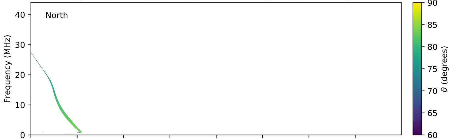
expres_earth_jupiter_io_jrm09_lossc-wid1deg_3kev_20060208_v01.cdf
