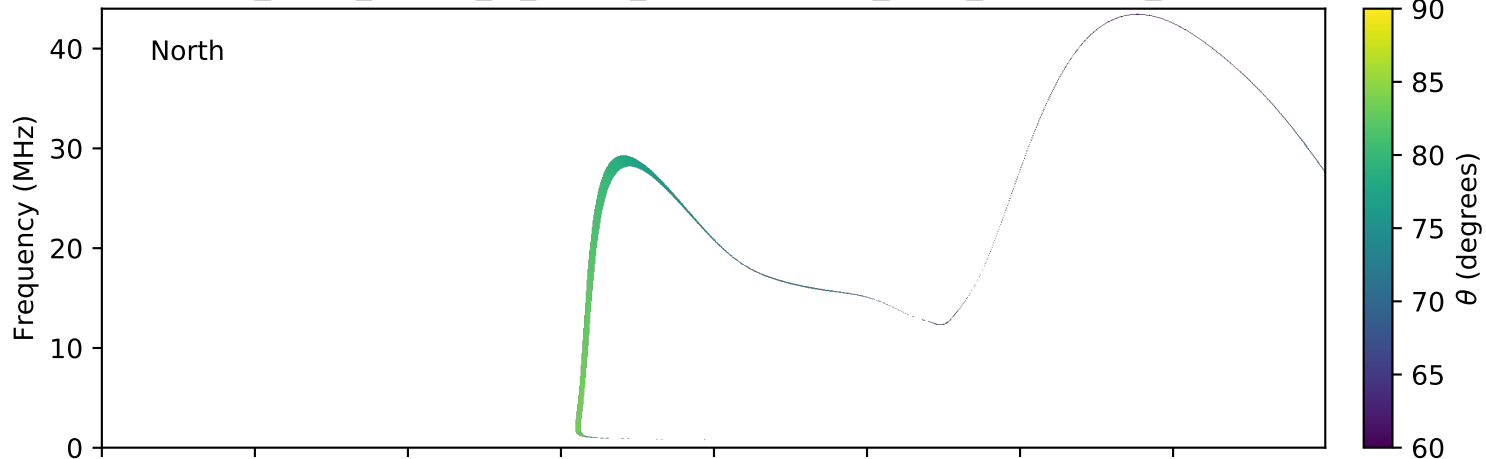
expres_earth_jupiter_io_jrm09_lossc-wid1deg_3kev_20060207_v01.cdf
