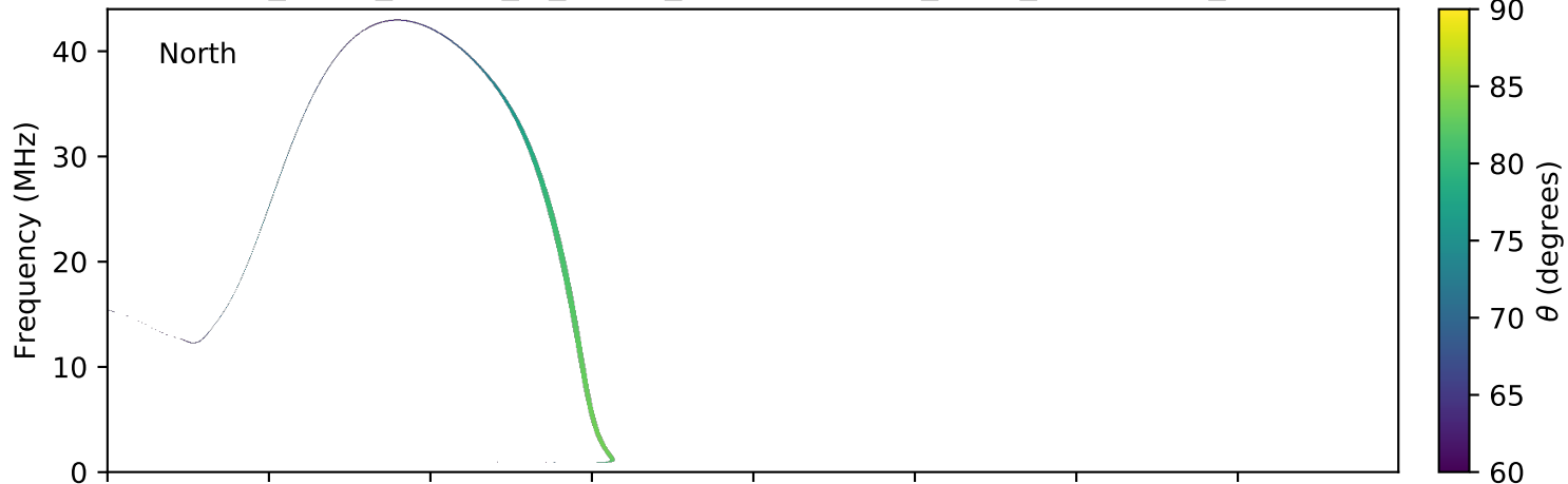
expres_earth_jupiter_io_jrm09_lossc-wid1deg_3kev_20060206_v01.cdf
