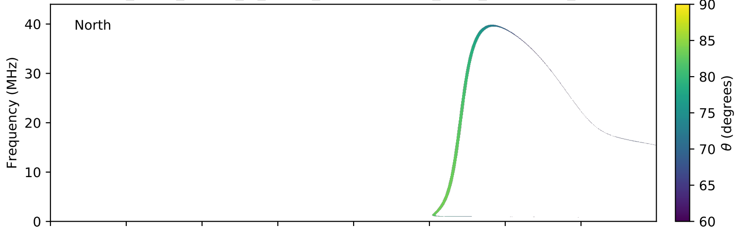
expres_earth_jupiter_io_jrm09_lossc-wid1deg_3kev_20060205_v01.cdf
