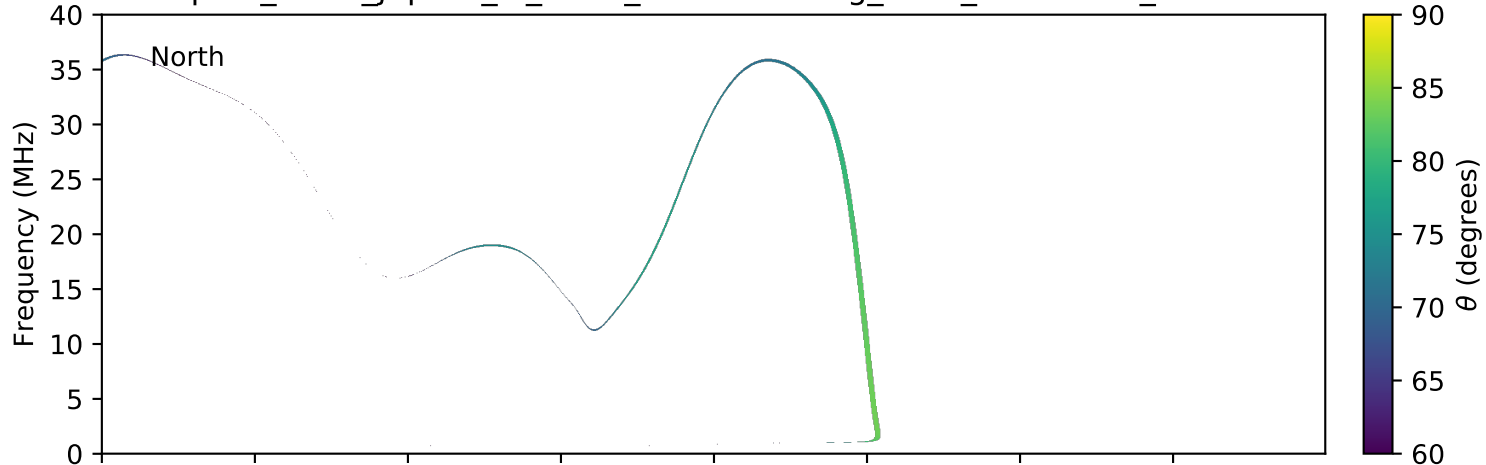
expres_earth_jupiter_io_isaac_lossc-wid1deg_3kev_20060227_v01.cdf
