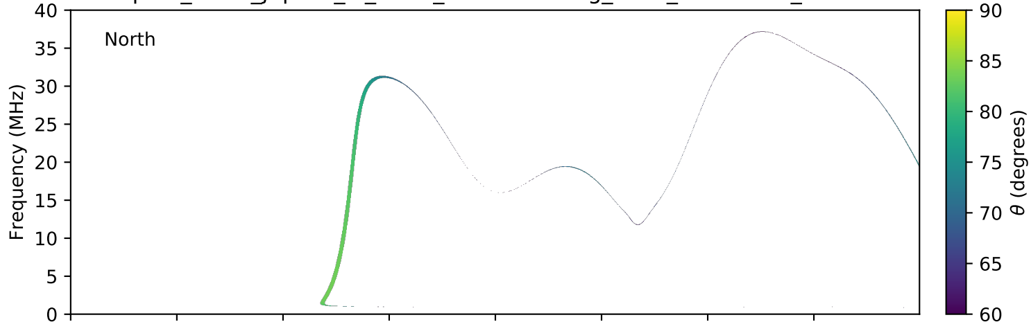
expres_earth_jupiter_io_isaac_lossc-wid1deg_3kev_20060223_v01.cdf
