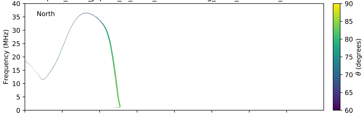
expres_earth_jupiter_io_isaac_lossc-wid1deg_3kev_20060222_v01.cdf
