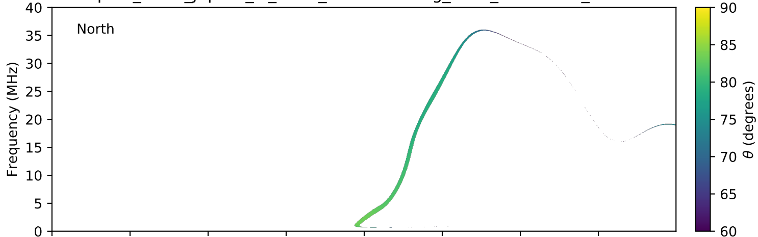
expres_earth_jupiter_io_isaac_lossc-wid1deg_3kev_20060221_v01.cdf
