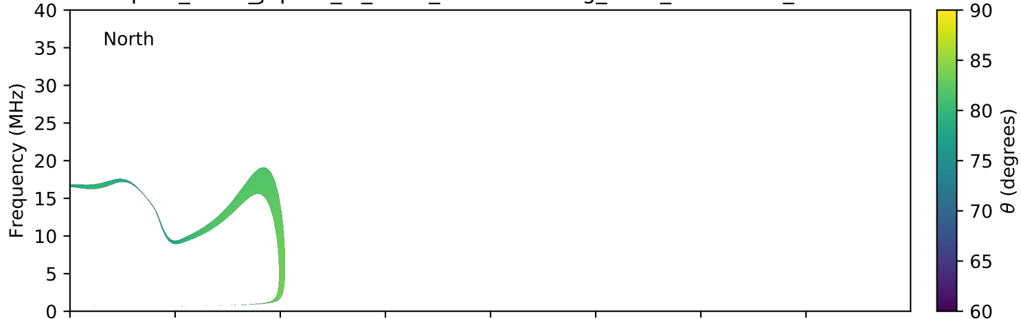
expres_earth_jupiter_io_isaac_lossc-wid1deg_3kev_20060215_v01.cdf
