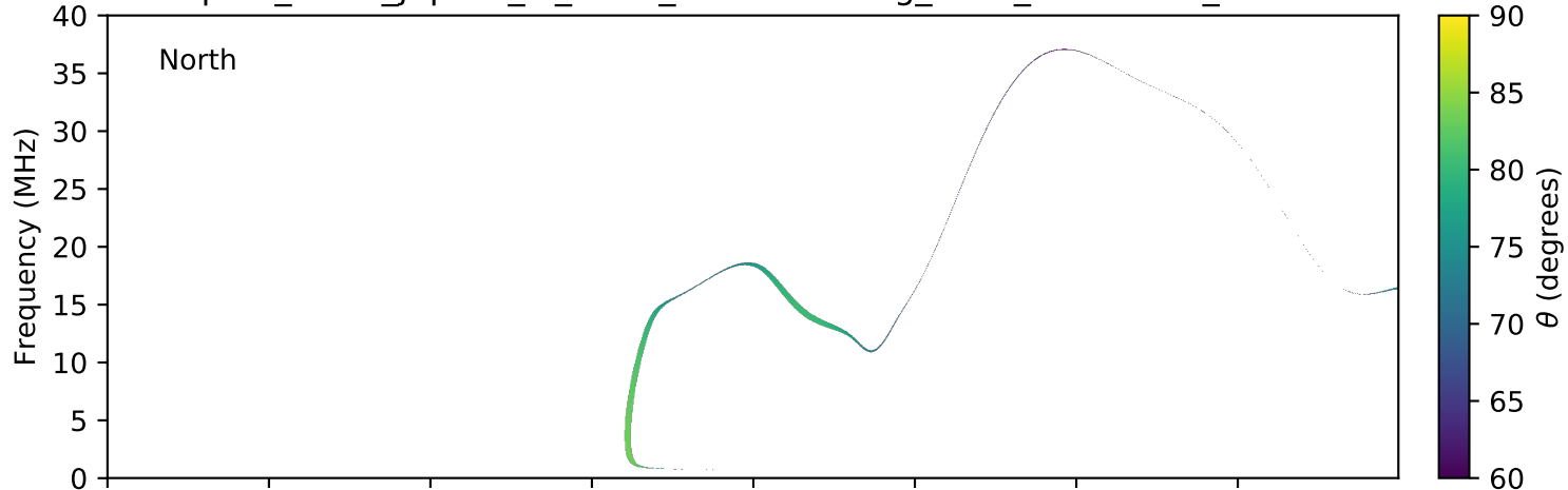
expres_earth_jupiter_io_isaac_lossc-wid1deg_3kev_20060214_v01.cdf
