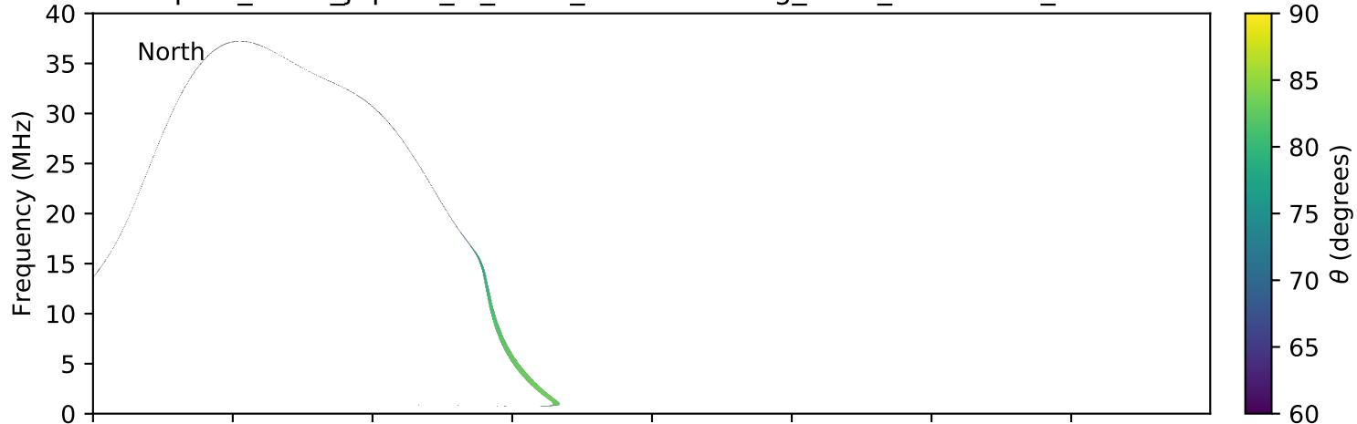
expres_earth_jupiter_io_isaac_lossc-wid1deg_3kev_20060213_v01.cdf
