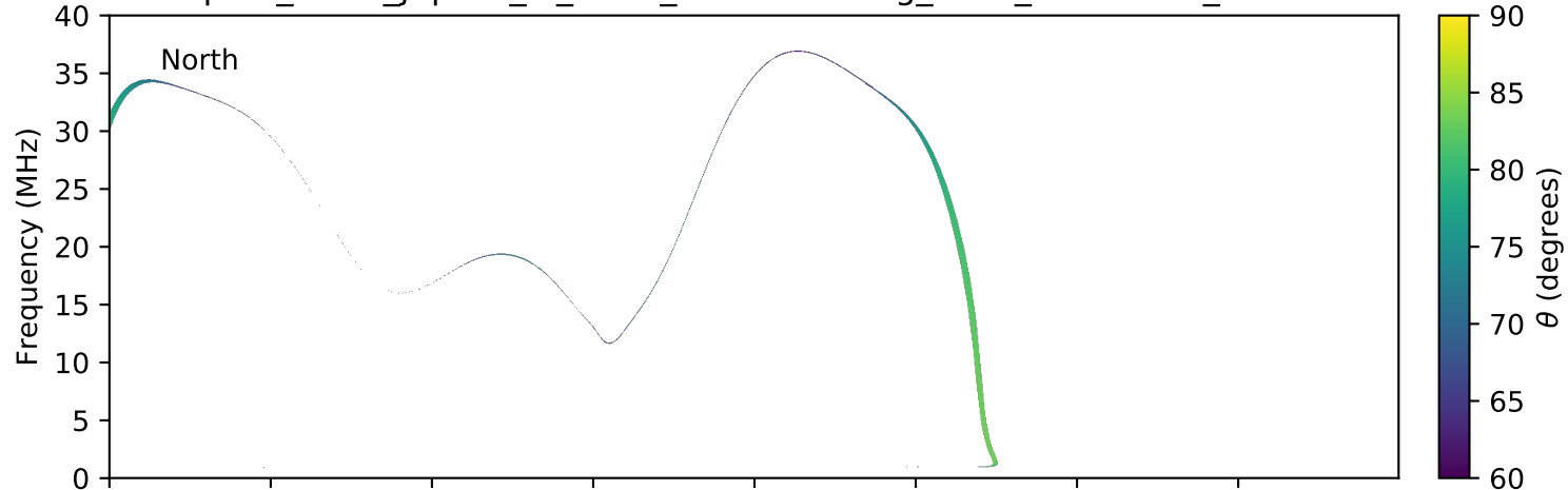
expres_earth_jupiter_io_isaac_lossc-wid1deg_3kev_20060211_v01.cdf
