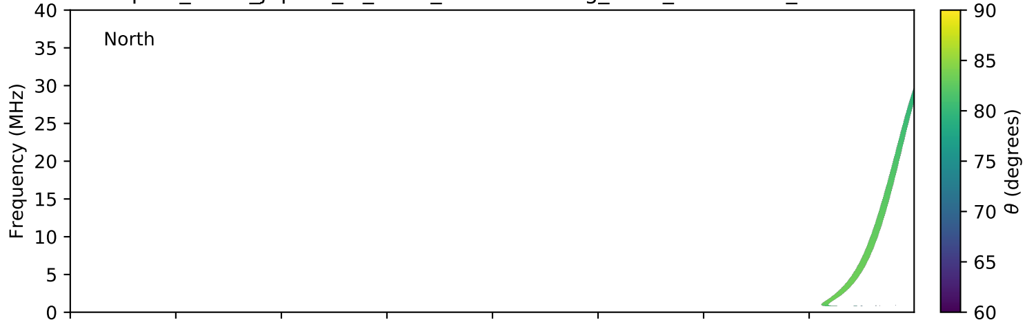
expres_earth_jupiter_io_isaac_lossc-wid1deg_3kev_20060210_v01.cdf
