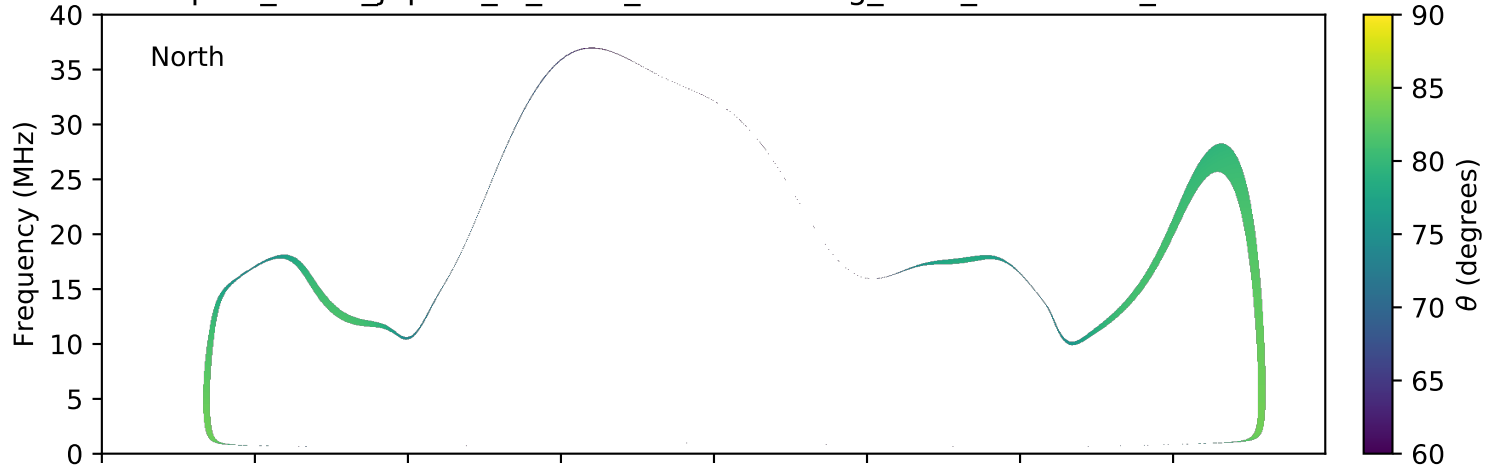
expres_earth_jupiter_io_isaac_lossc-wid1deg_3kev_20060209_v01.cdf
