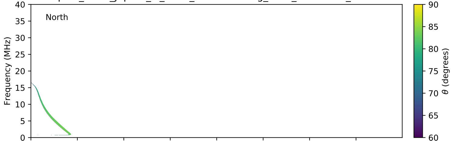
expres_earth_jupiter_io_isaac_lossc-wid1deg_3kev_20060208_v01.cdf
