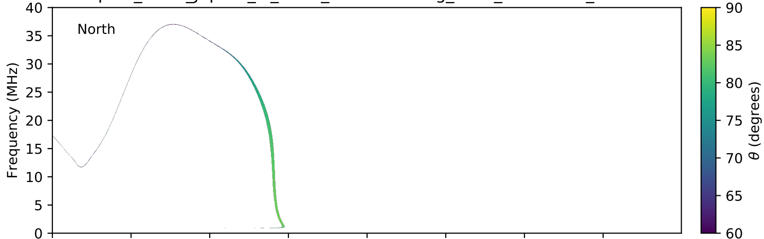
expres_earth_jupiter_io_isaac_lossc-wid1deg_3kev_20060206_v01.cdf
