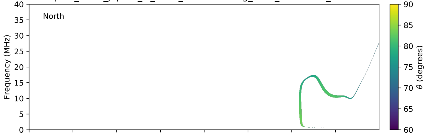
expres_earth_jupiter_io_isaac_lossc-wid1deg_3kev_20060203_v01.cdf
