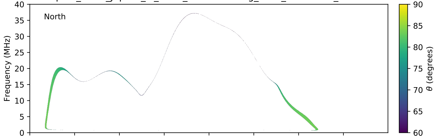
expres_earth_jupiter_io_isaac_lossc-wid1deg_3kev_20060202_v01.cdf
