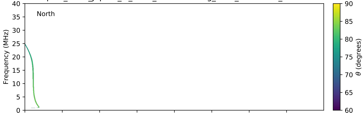
expres_earth_jupiter_io_isaac_lossc-wid1deg_3kev_20060201_v01.cdf
