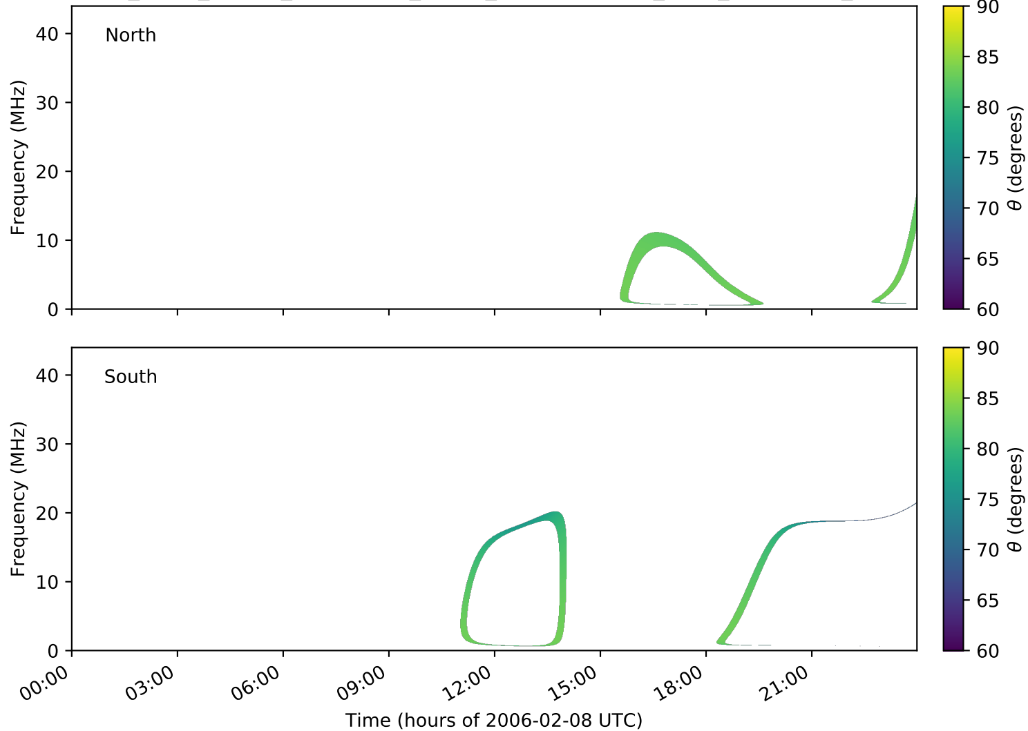
expres_earth_jupiter_ganymede_jrm09_lossc-wid1deg_3kev_20060208_v01.cdf
