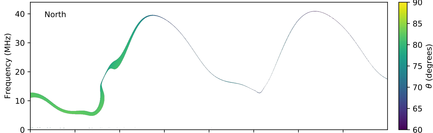
expres_earth_jupiter_europa_jrm09_lossc-wid1deg_3kev_20060224_v01.cdf
