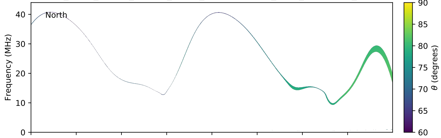
expres_earth_jupiter_europa_jrm09_lossc-wid1deg_3kev_20060221_v01.cdf
