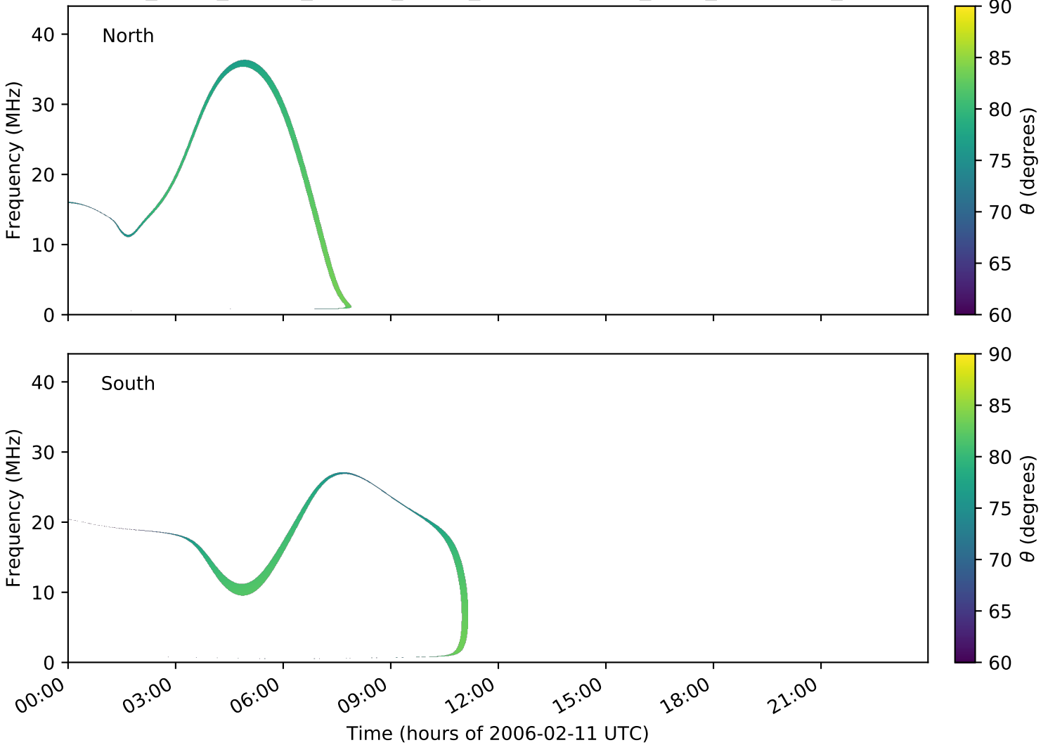
expres_earth_jupiter_europa_jrm09_lossc-wid1deg_3kev_20060211_v01.cdf
