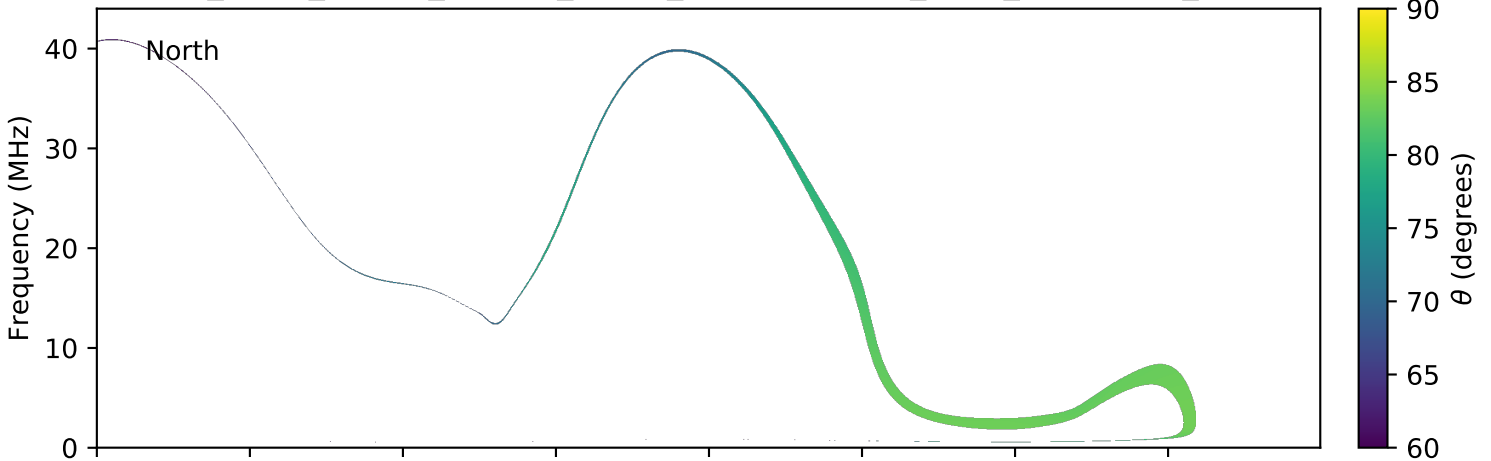
expres_earth_jupiter_europa_jrm09_lossc-wid1deg_3kev_20060207_v01.cdf
