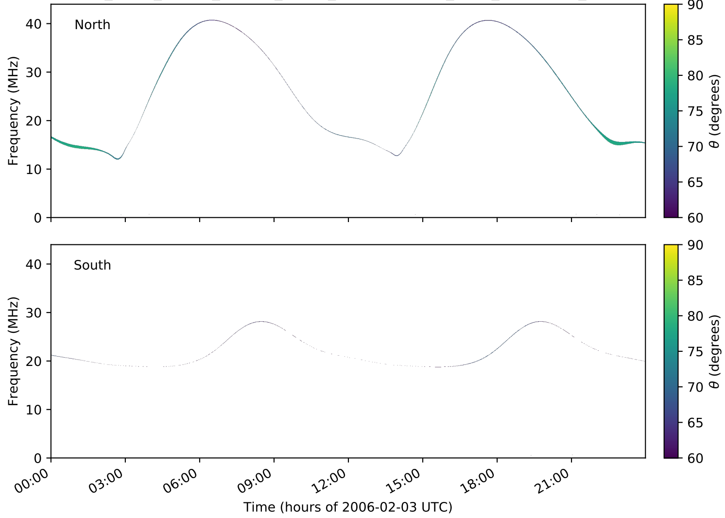
expres_earth_jupiter_europa_jrm09_lossc-wid1deg_3kev_20060203_v01.cdf
