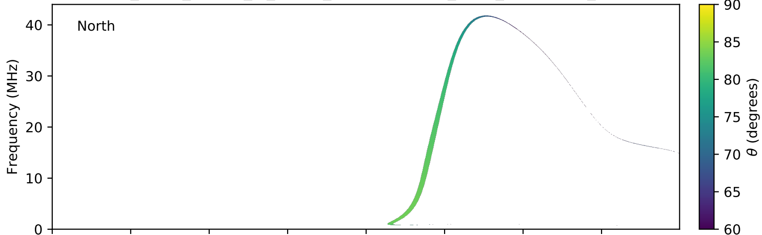
expres_earth_jupiter_io_jrm09_lossc-wid1deg_3kev_20060129_v01.cdf
