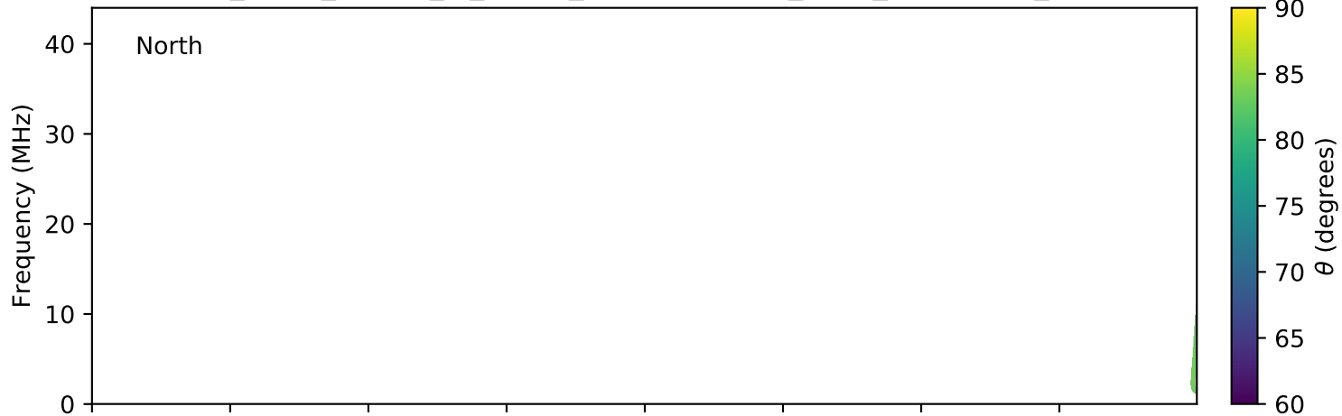
expres_earth_jupiter_io_jrm09_lossc-wid1deg_3kev_20060125_v01.cdf
