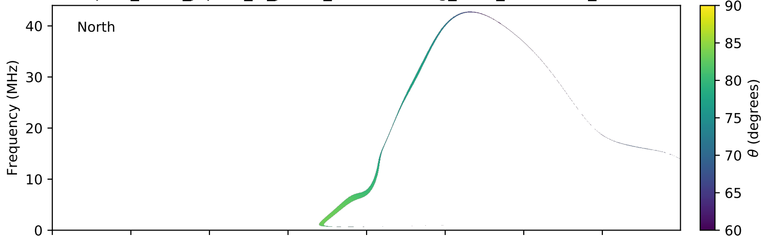
expres_earth_jupiter_io_jrm09_lossc-wid1deg_3kev_20060122_v01.cdf
