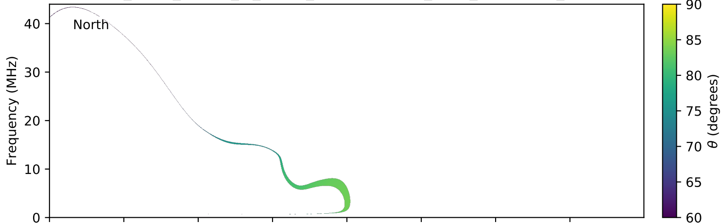
expres_earth_jupiter_io_jrm09_lossc-wid1deg_3kev_20060121_v01.cdf
