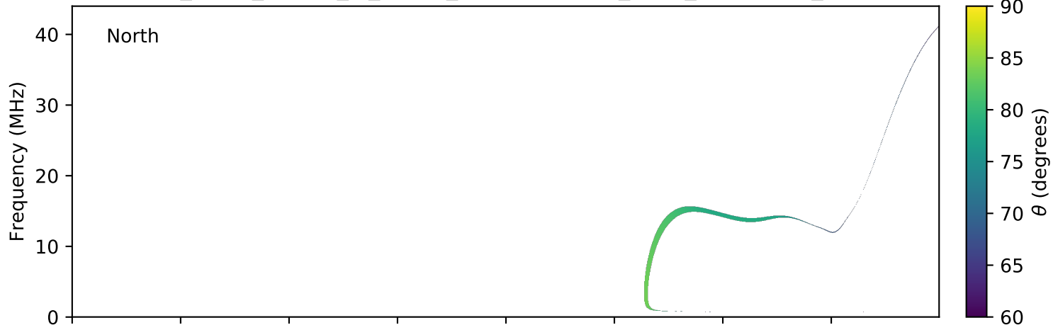
expres_earth_jupiter_io_jrm09_lossc-wid1deg_3kev_20060120_v01.cdf
