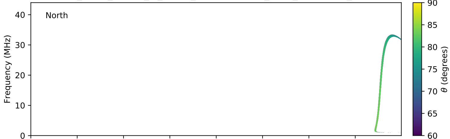
expres_earth_jupiter_io_jrm09_lossc-wid1deg_3kev_20060118_v01.cdf
