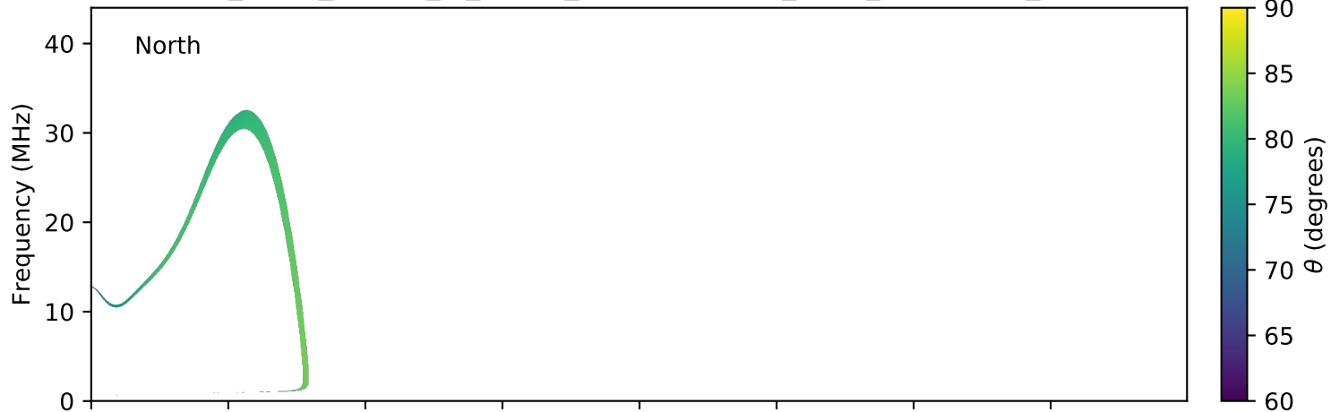
expres_earth_jupiter_io_jrm09_lossc-wid1deg_3kev_20060116_v01.cdf
