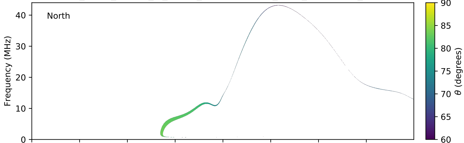
expres_earth_jupiter_io_jrm09_lossc-wid1deg_3kev_20060115_v01.cdf
