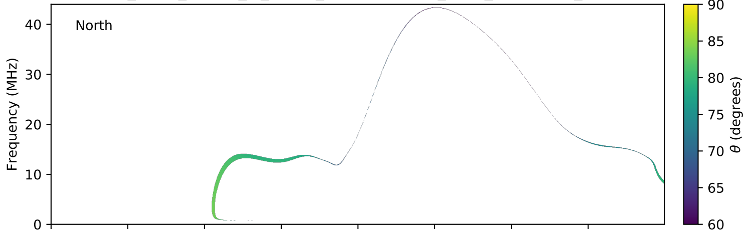
expres_earth_jupiter_io_jrm09_lossc-wid1deg_3kev_20060108_v01.cdf
