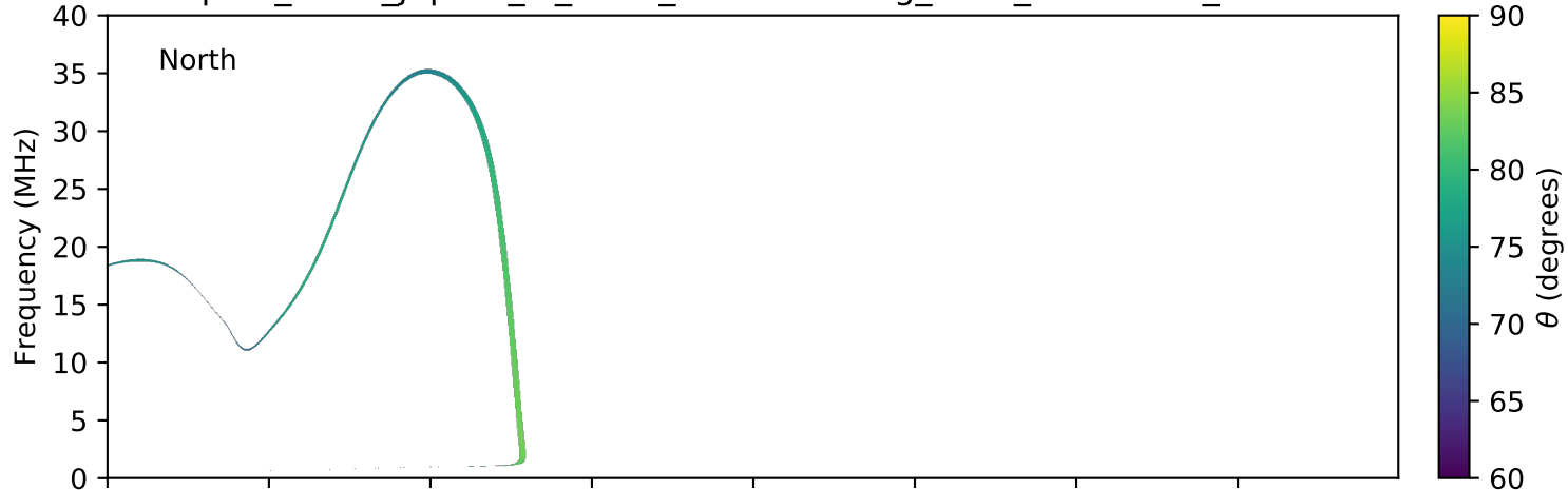
expres_earth_jupiter_io_isaac_lossc-wid1deg_3kev_20060130_v01.cdf
