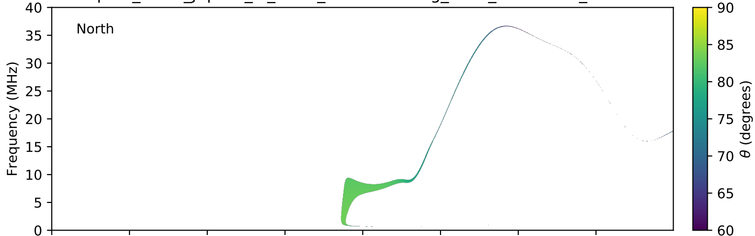
expres_earth_jupiter_io_isaac_lossc-wid1deg_3kev_20060129_v01.cdf
