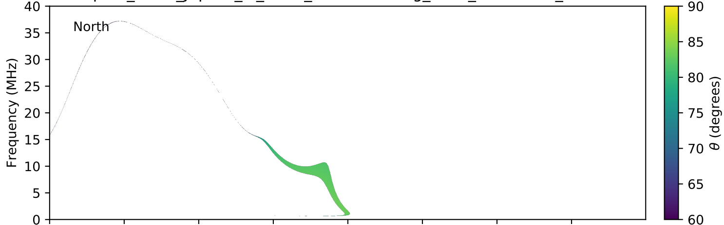
expres_earth_jupiter_io_isaac_lossc-wid1deg_3kev_20060128_v01.cdf
