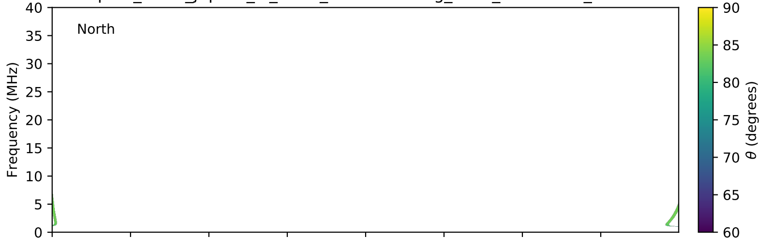
expres_earth_jupiter_io_isaac_lossc-wid1deg_3kev_20060125_v01.cdf
