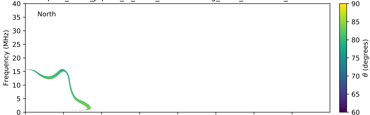
expres_earth_jupiter_io_isaac_lossc-wid1deg_3kev_20060123_v01.cdf
