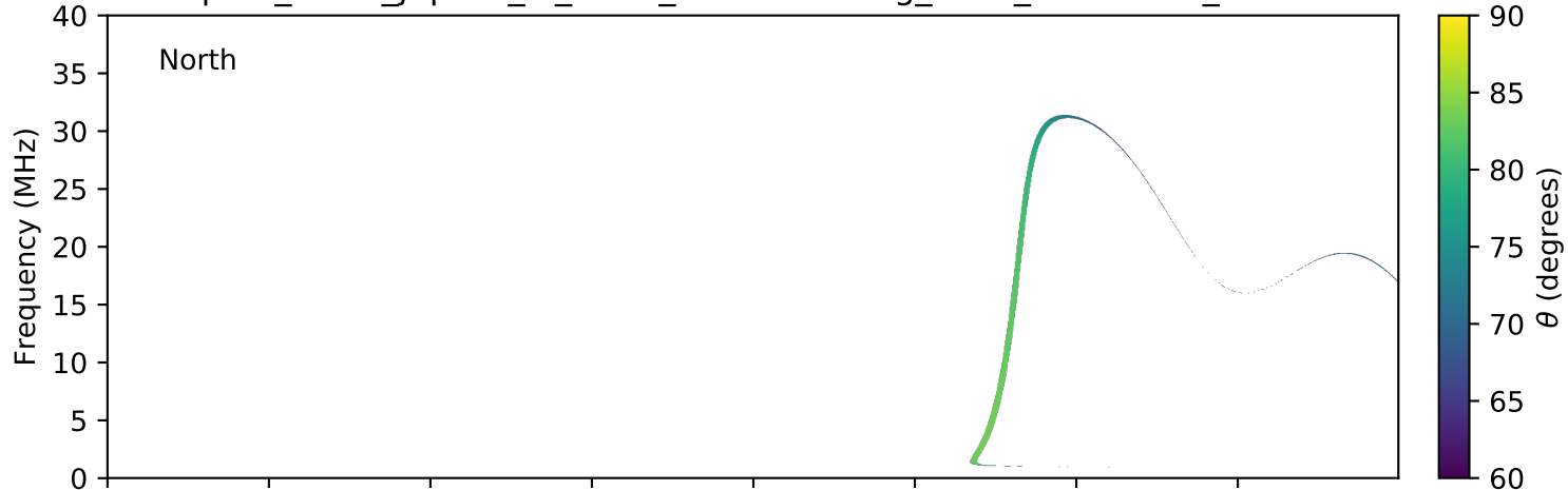
expres_earth_jupiter_io_isaac_lossc-wid1deg_3kev_20060120_v01.cdf
