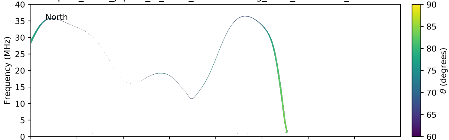
expres_earth_jupiter_io_isaac_lossc-wid1deg_3kev_20060119_v01.cdf
