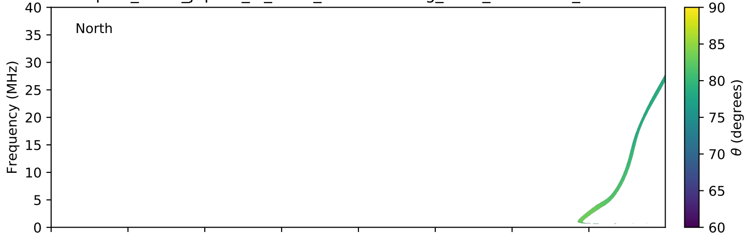
expres_earth_jupiter_io_isaac_lossc-wid1deg_3kev_20060118_v01.cdf
