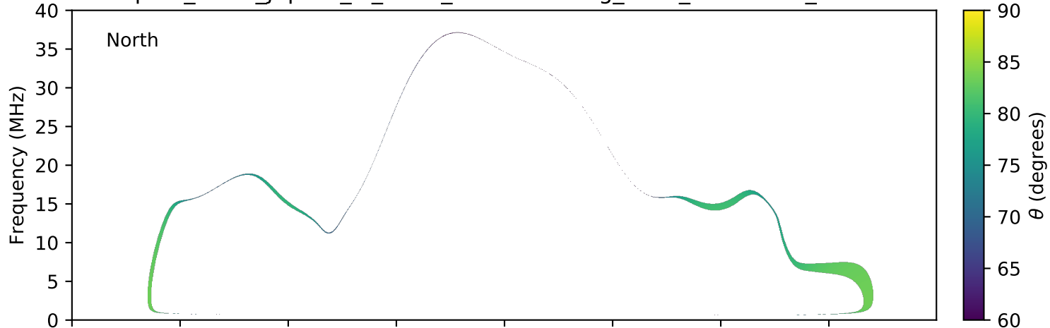
expres_earth_jupiter_io_isaac_lossc-wid1deg_3kev_20060117_v01.cdf
