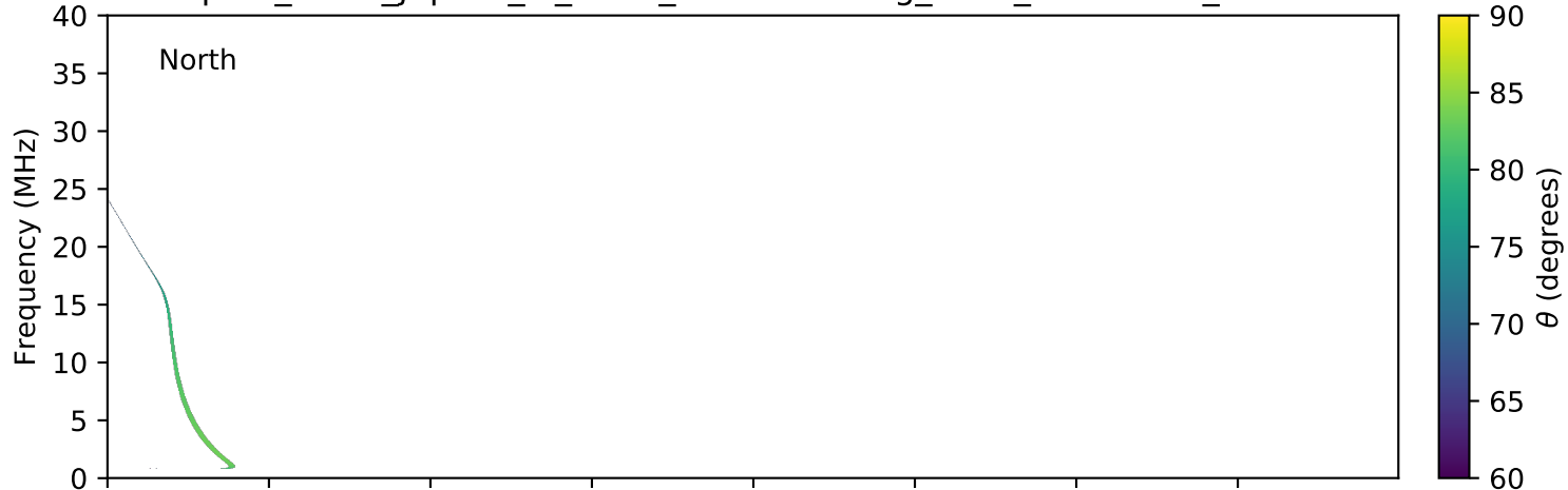
expres_earth_jupiter_io_isaac_lossc-wid1deg_3kev_20060116_v01.cdf
