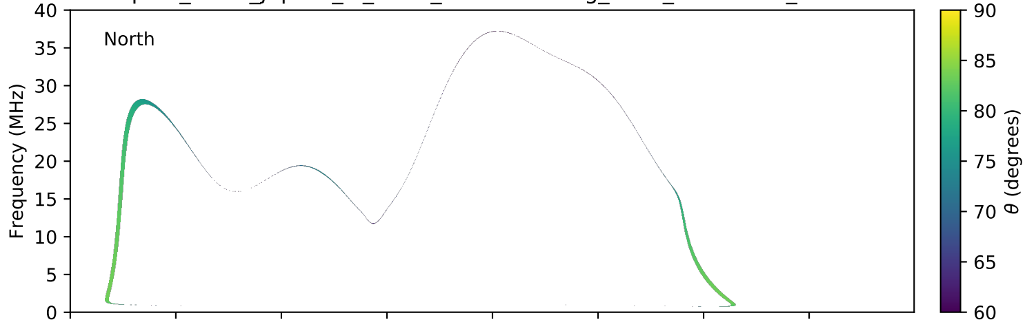
expres_earth_jupiter_io_isaac_lossc-wid1deg_3kev_20060110_v01.cdf
