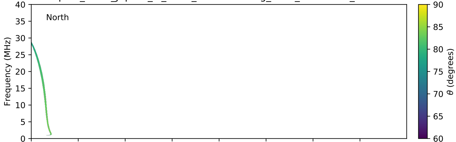
expres_earth_jupiter_io_isaac_lossc-wid1deg_3kev_20060109_v01.cdf
