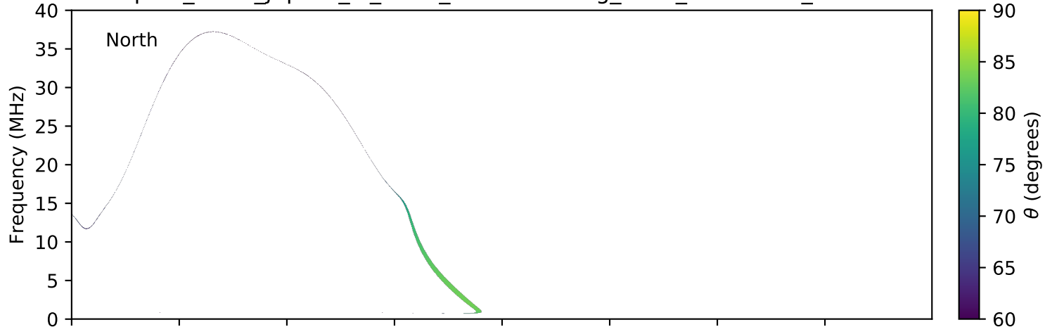
expres_earth_jupiter_io_isaac_lossc-wid1deg_3kev_20060105_v01.cdf
